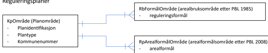
Figur : Datamodell for reguleringsplaner
